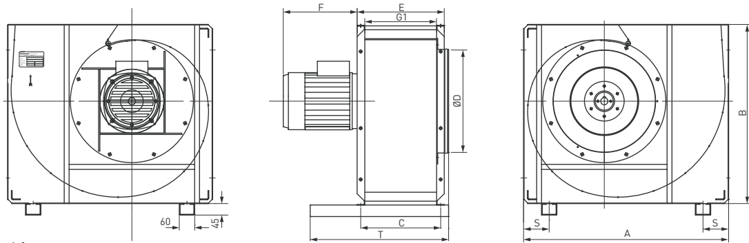
Directly coupled fans
