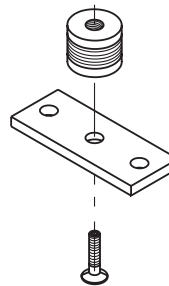
Base plate for anti-vibration mountings
