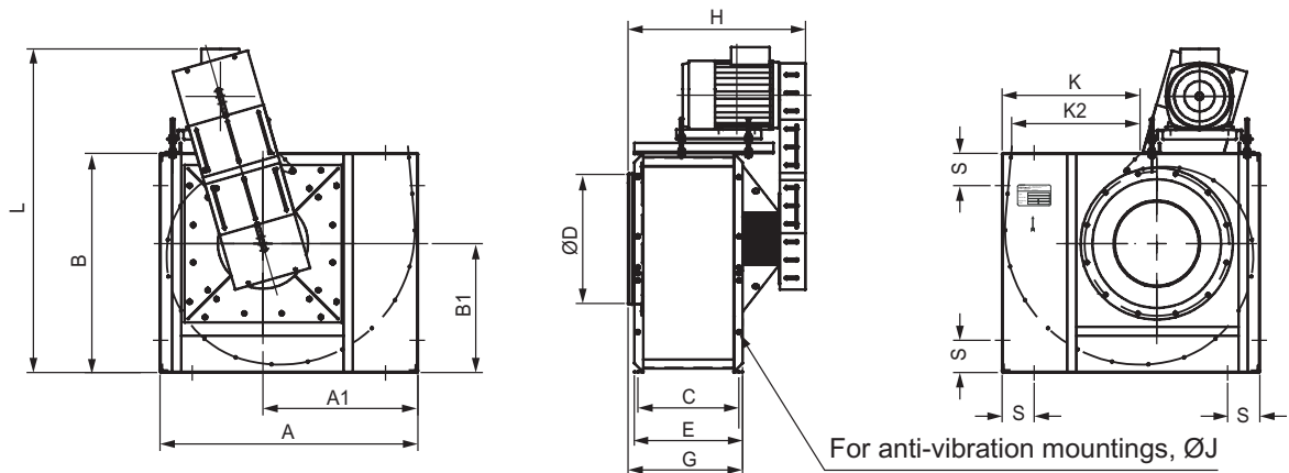
Belt-driven fans
